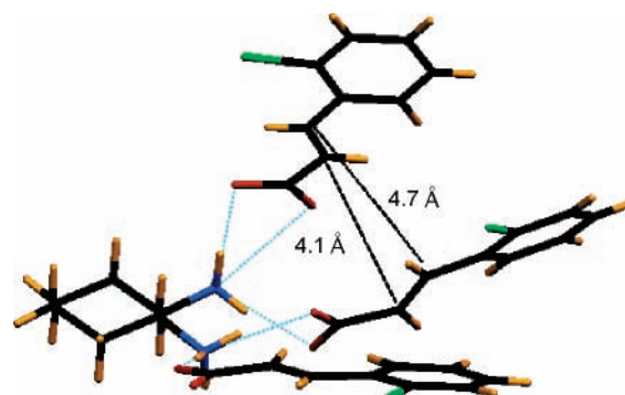
Figure 4. Crystal structure of salt 2 showing three closely lying cinnamate molecules hydrogen bonded to the trans -1,2-diaminocyclohexane moiety; only the closely lying cinnamate pair alkene–alkene distances are shown.
