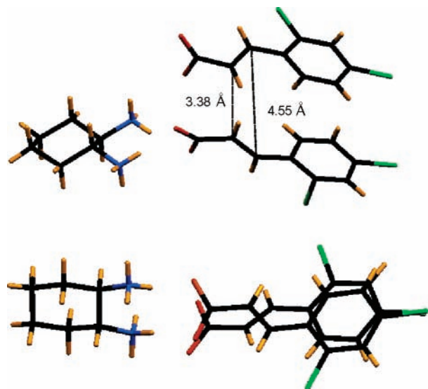
Figure 2. (a) Crystal structure of diamine double salt 1 showing alkene distances. (b) Crystal structure of salt 1 viewed along the “a” axis showing a crisscross alignment of olefins.
