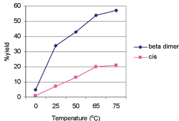
Figure 3. Temperature dependence of the cis isomer and cyclobutane from salt of 1 . The salt was photolyzed for the same duration (20 h) at all temperatures.
